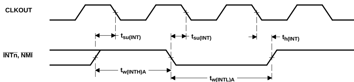
Figure 4-15. Interrupt Timing
