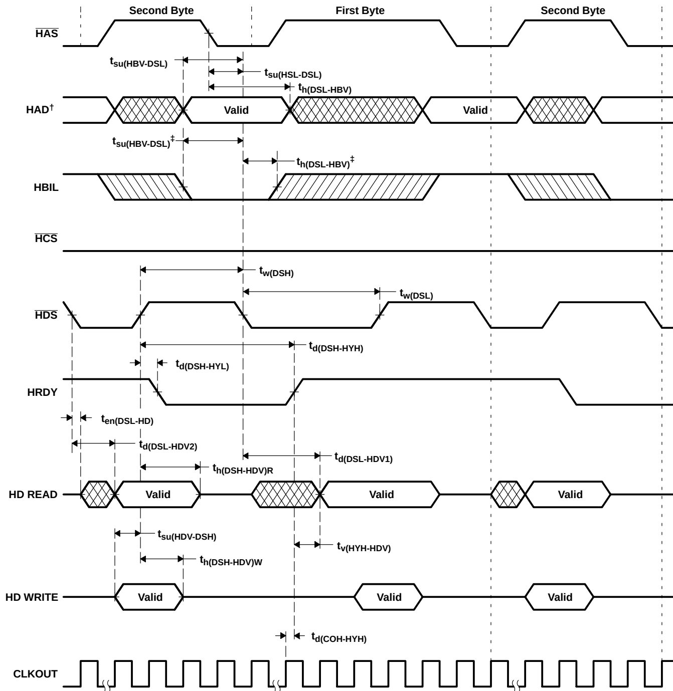
Figure 4-27. Using HDS to Control Accesses ( \overline{HCS} Always Low)
