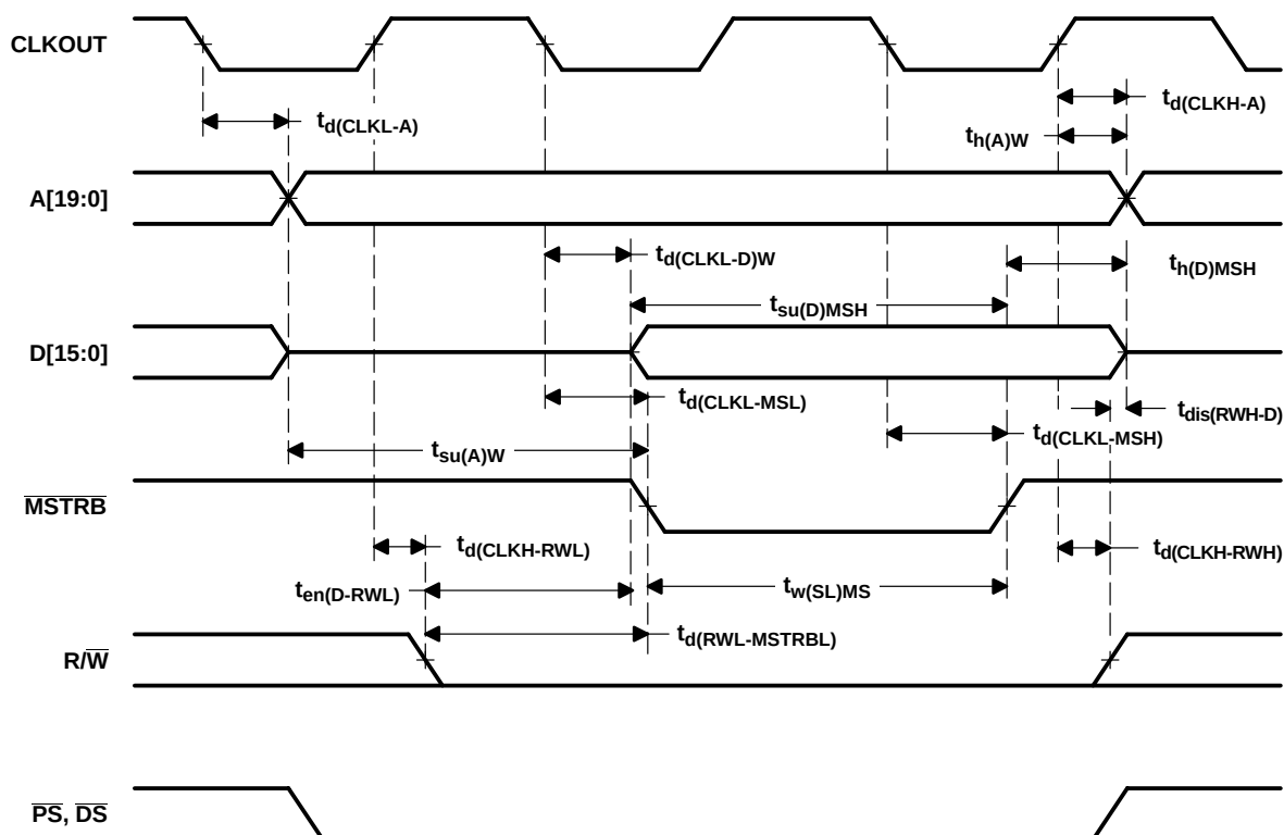
Figure 4–6. Memory Write ( \overline{\text{MSTRB}} = 0 )
